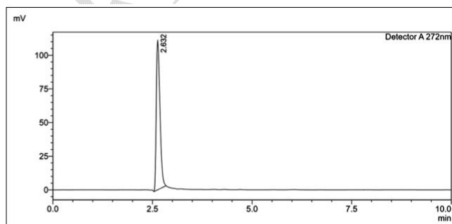
Figure 3: Chromatogram of standard gallic acid at 272 nm
