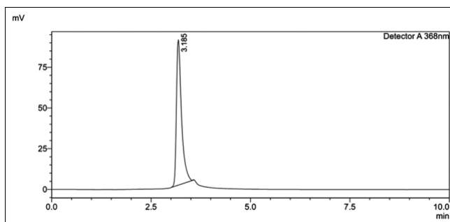
Figure 4: Chromatogram of standard kaempferol at 368 nm
