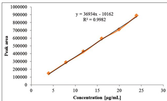
Figure 1: Standard calibration graph of gallic acid
