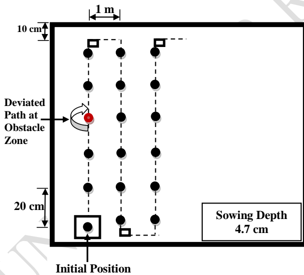
Figure1. Workspace of the Agrirobot
