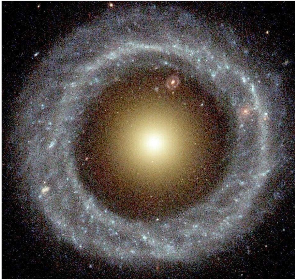
Fig.13.RingsaroundtheGalaxy
