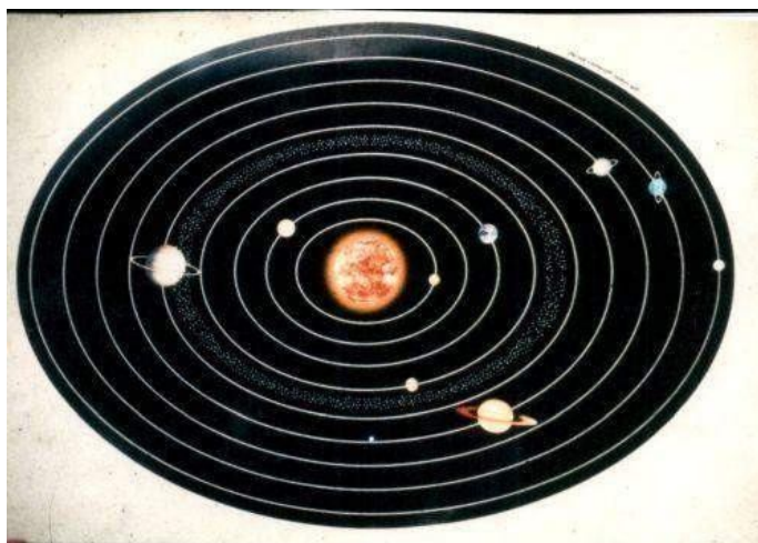
Fig.1. The solar system
