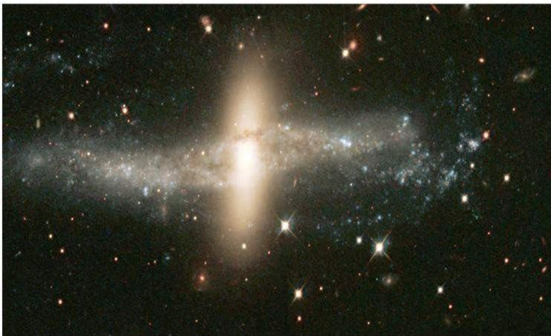
Fig.11.Ringsaroundthegalaxy
