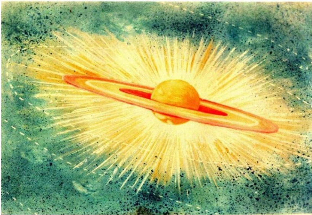
Fig.15.RingsaroundtheSun Table
