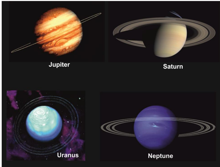
Fig. 9. Rings around the Planets
