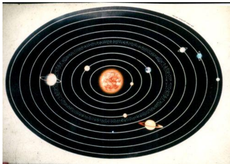
Fig. 2. The solar system
