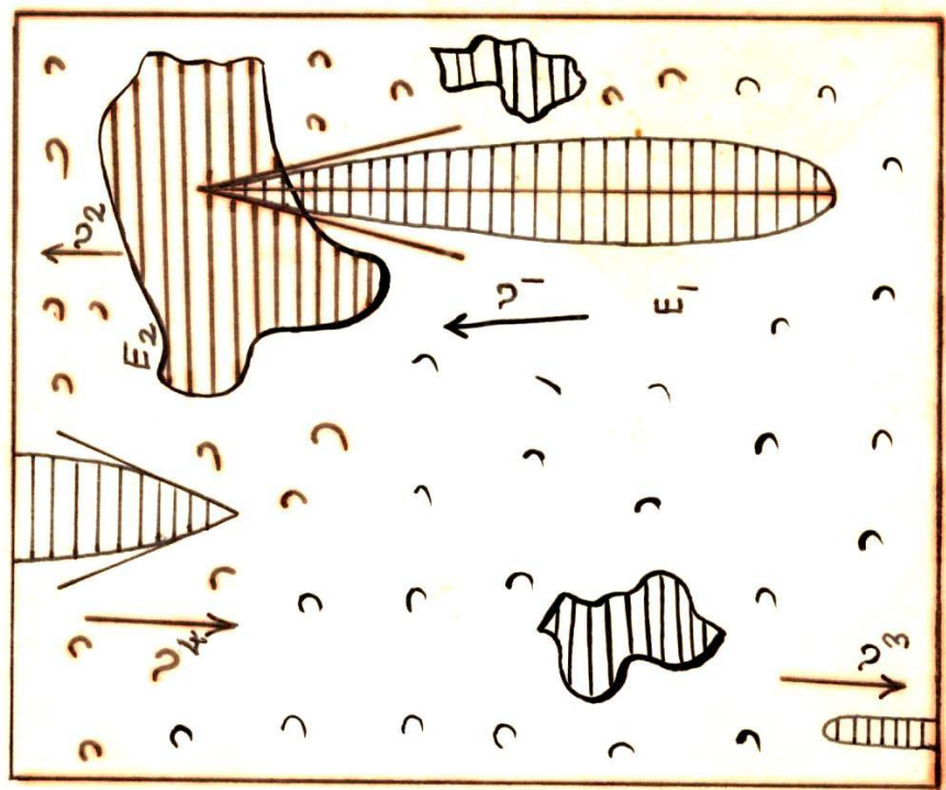
Fig. 3. Supersonic turbulent convection
