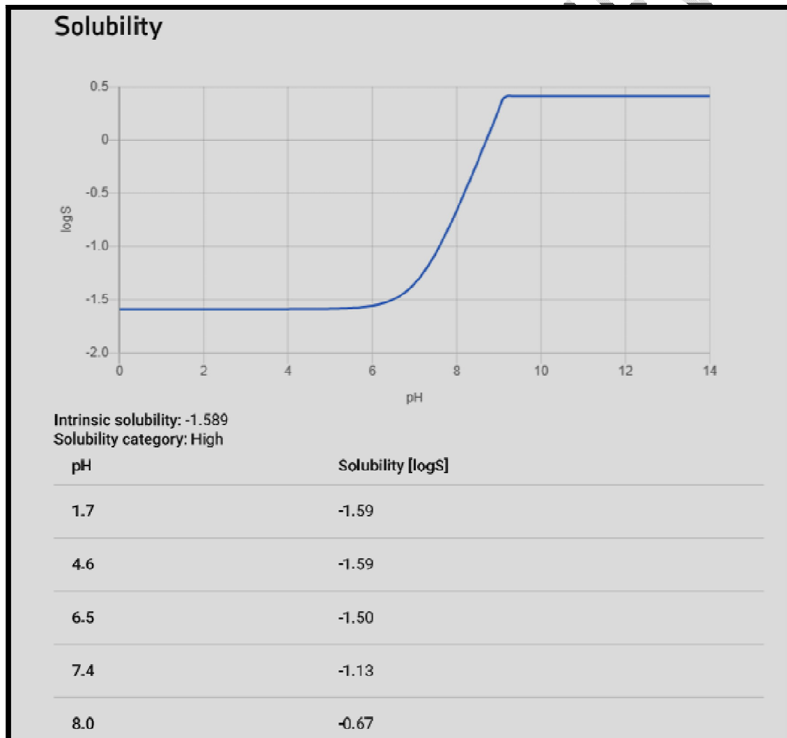
Fig.5 Distribution of log S with pH of Indoline-2,3-dione-3-oxime as given by chemicalize software
