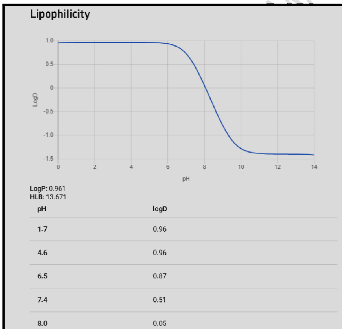
Fig.4 Distribution of log D with pH of Indoline-2,3-dione-3-oxime as given by chemicalize software
