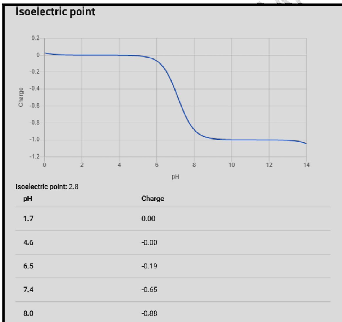
Fig.3 Distribution of charge with pH of Indoline-2,3-dione-3-oxime as given by chemicalize software
