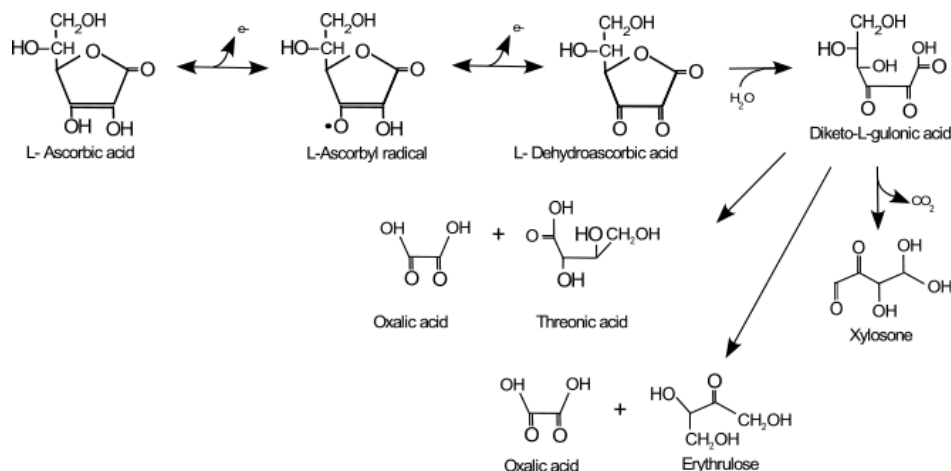
Figure 1. Vitamin C metabolism. In humans, AA is oxidized and degraded into 2–4 carbon products. Translated and modified from Villagrán et al. [9].
